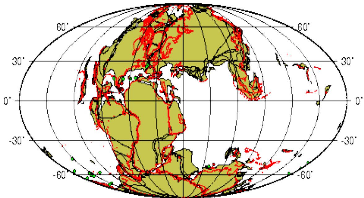
150 My Reconstruction
